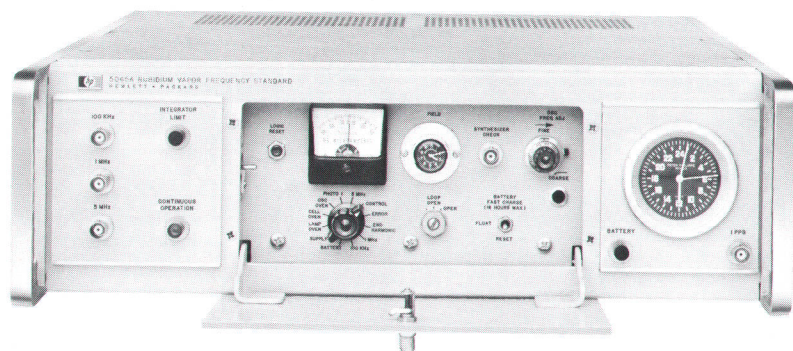
Fig. 1. New rubidium-type frequency standard provides high-stability output signal for use in precision frequency work.
